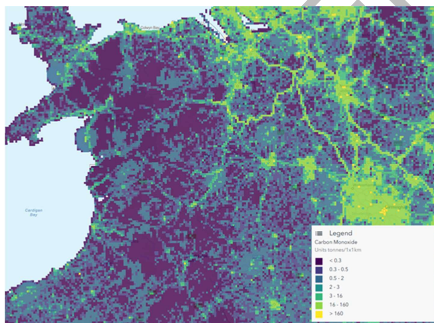
Ffigur B-5-6: Crynodiadau Carbon Monocsid ar draws Eryri
